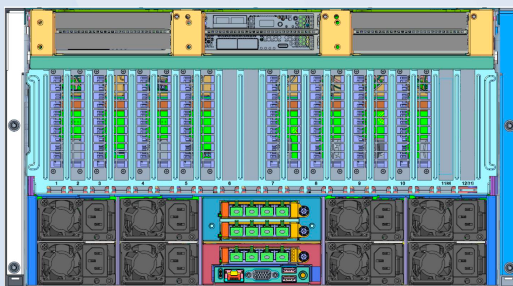
Rear View
